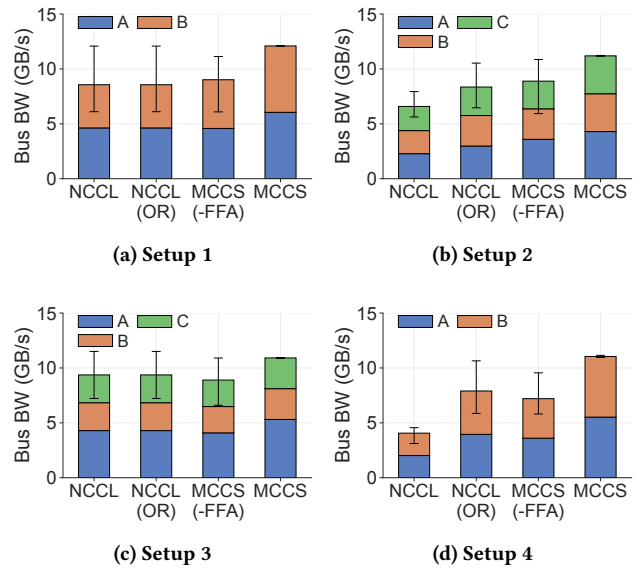
Figure 8: [Multi applications]: Application bus bandwidth. Error bars represent 95% percentile intervals.
