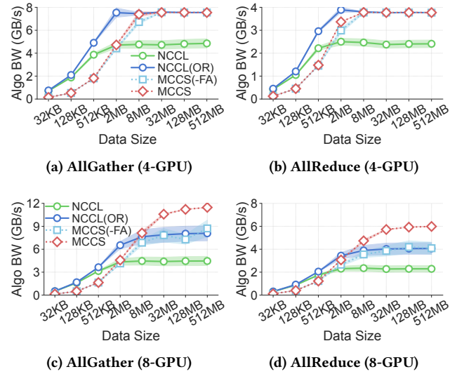
Figure 6: [Single application]: Algorithm bandwidth of AllReduce and AllGather. The shaded areas represent 95% percentile intervals.
